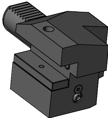
STRAIGHT VDI30 STATIC TOOL OUTPUT: 20mm SQR SHANK COOLANT: EXTERNAL
